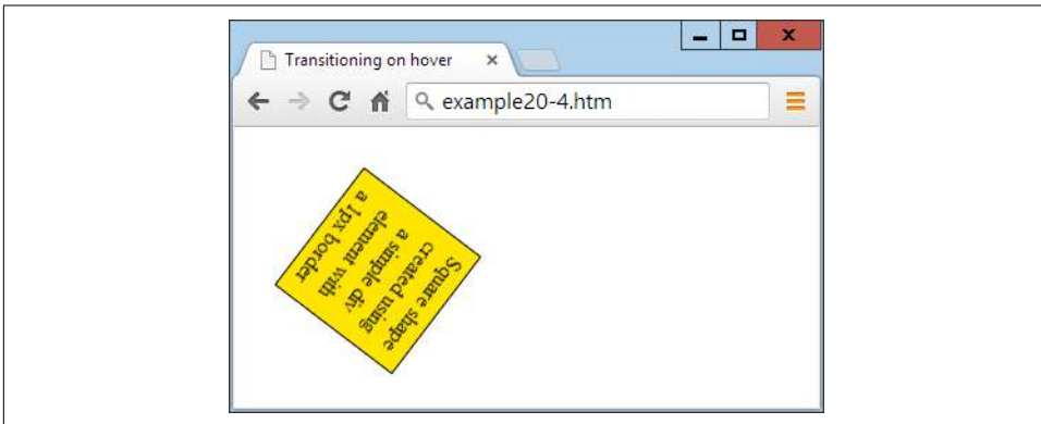
Figure 19-14. The object rotates and changes color when hovered over
