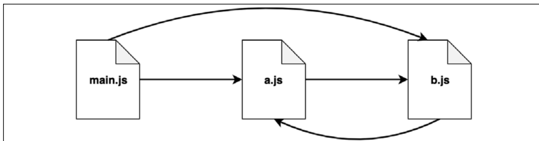
Figure 2.3: An example scenario with circular dependencies
