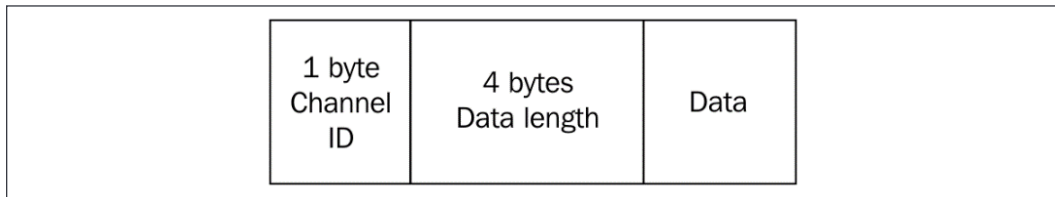
Figure 6.10: Bytes structure of the data packet for our remote logger
